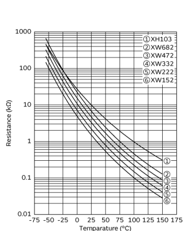
Resistance-Temperature Characteristics
